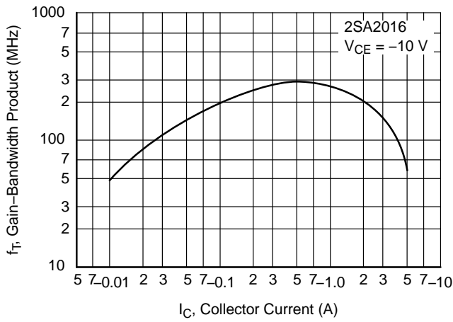
Figure 16. f T - I C
