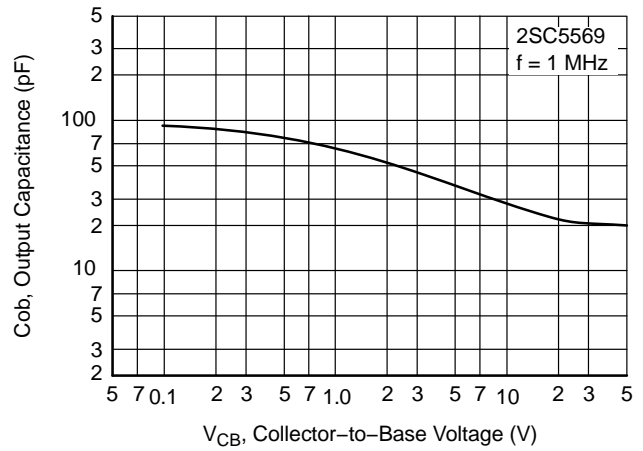
Figure 15. Cob - V CB
