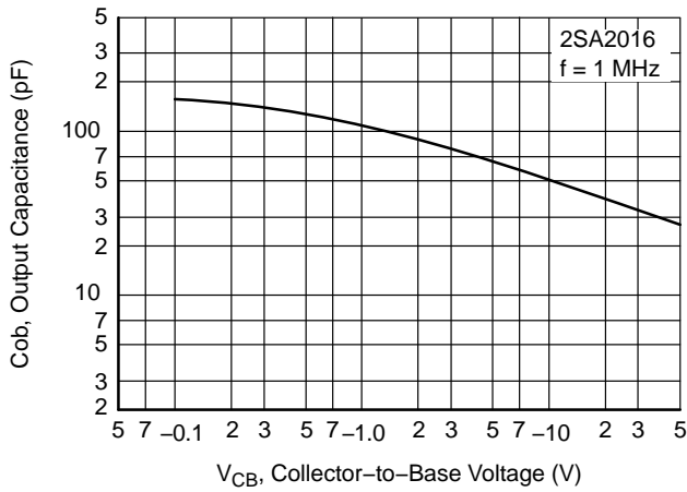
Figure 14. Cob - V CB
