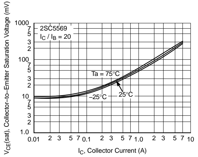
Figure 9. V_{CE(sat)} - I_C
