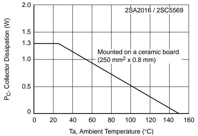
Figure 19. P C - T a
