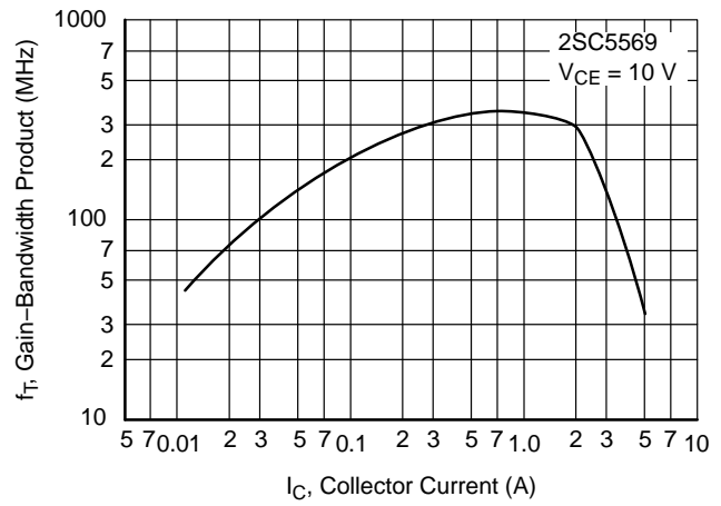
Figure 17. f T - I C
