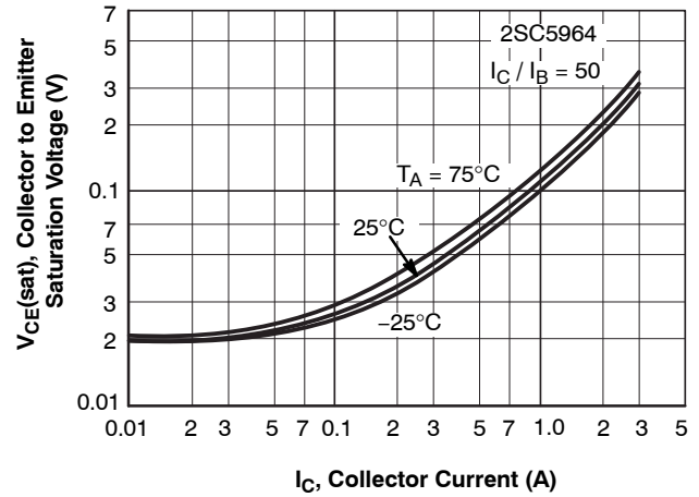
Figure 15. V_{CE(sat)} - I_C
