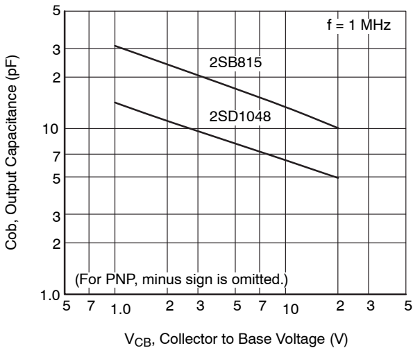
Figure 6. C_{ob} - V_{CB}
