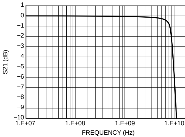
Figure 12. Typical Insertion Loss
