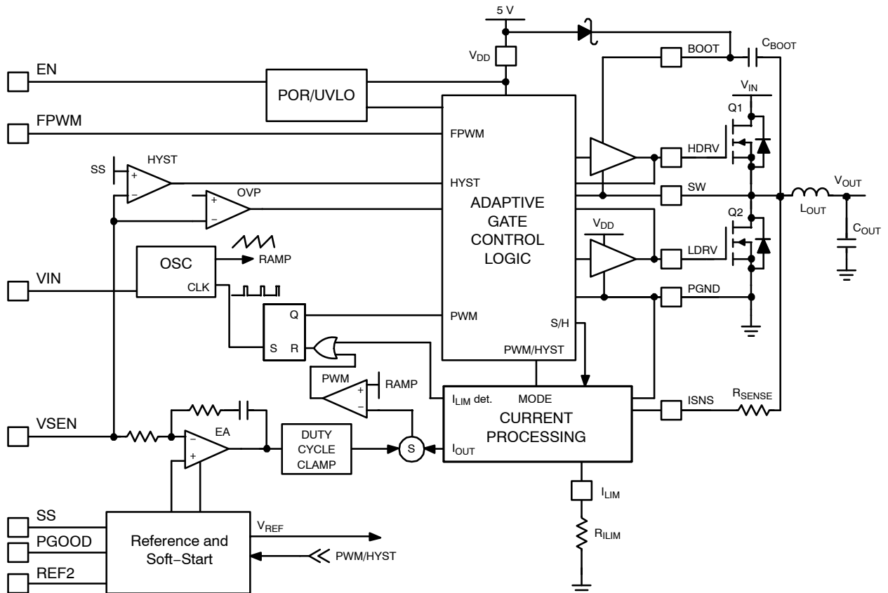
Figure 2. Block Diagram
