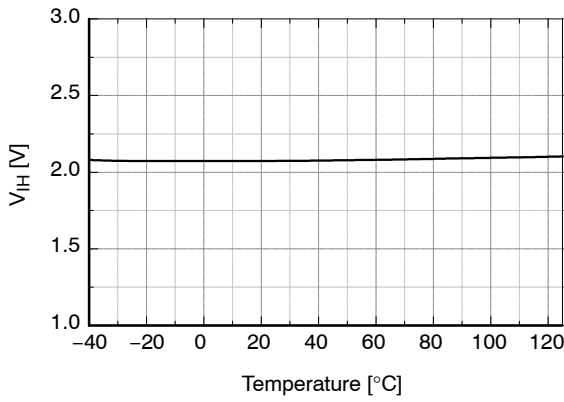
Figure 24. Logic HIGH Input Voltage vs. Temperature
