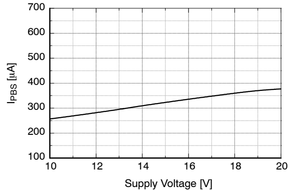
Figure 33. Operating V BS Supply Current vs. Supply Voltage
