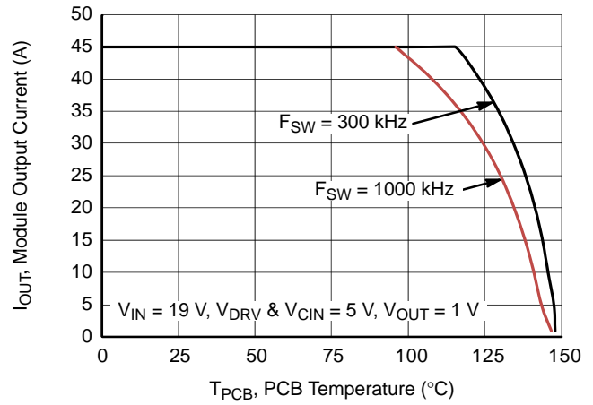
Figure 6. Safe Operating Area for 19 V_{IN}
