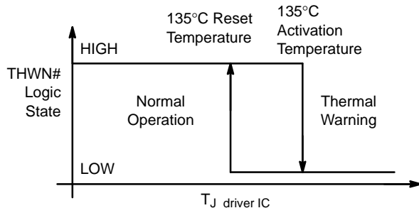
Figure 27. THWN Operation
