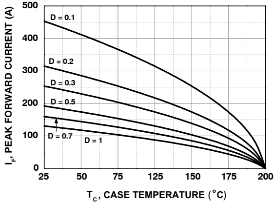
Figure 3. Current Derating
