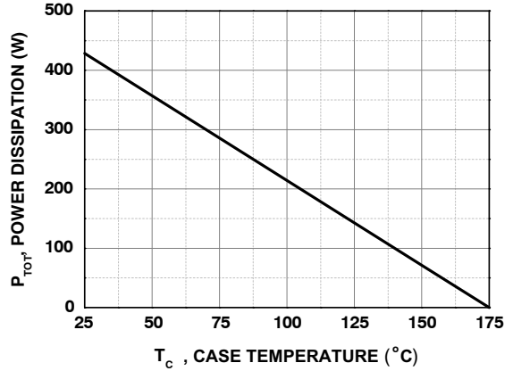
Figure 4. Power Derating
