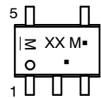
SC-88A / SOT-353 / SC-70 DF SUFFIX CASE 419A-02
