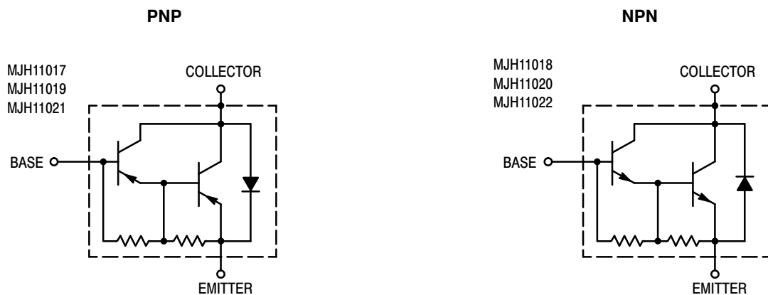
Figure 9. Darlington Schematic
