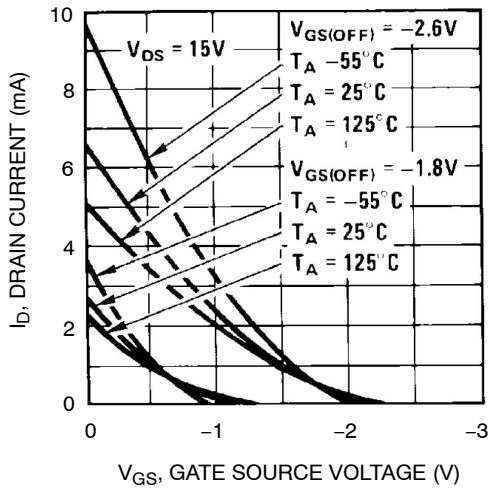
Figure 1. Transfer Characteristics
