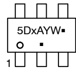
TSOP-6 (SOT23-6) SN SUFFIX CASE 318G STYLE 13
