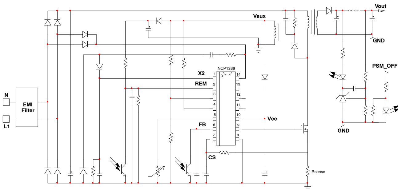
Figure 1. NCP1339 Typical Application Circuit (without IFF pin)
