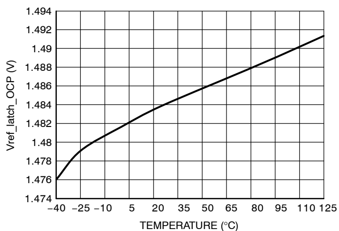
Figure 22. OCP Latch Reference ( V_{ref\_latch\_OCP} )
