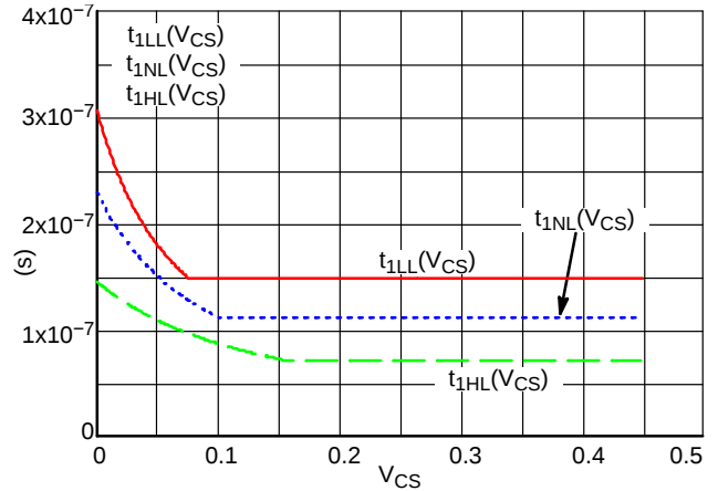
Figure 61. The Dead Time Evolution with Input Voltage and the Sensed Current
