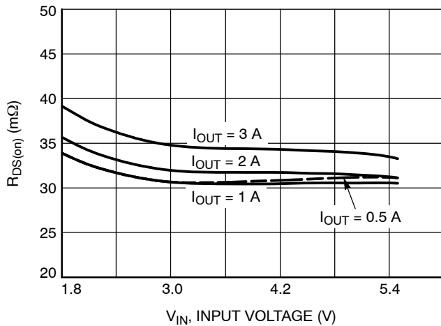
Figure 5. R_{DS(on)} vs. V_{IN} Voltage at 25^\circ\text{C}
