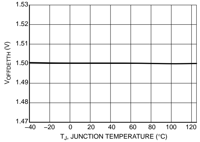
Figure 10. V_{OFFDETH} at V_{CC} = 15\text{ V}
