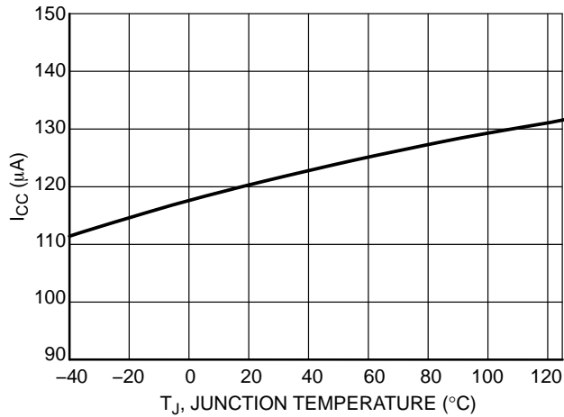
Figure 13. I_{CC} in Regulation at V_{CC} = 15\text{ V} for NCP4354A
