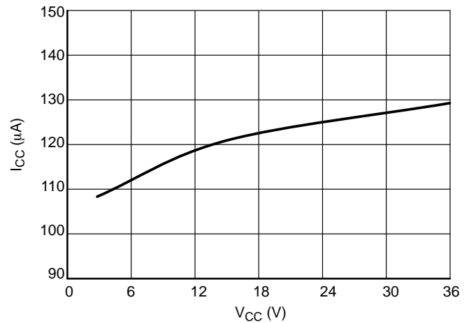
Figure 14. I_{CC} in Regulation at T_J = 25^{\circ}\text{C} for NCP4354A
