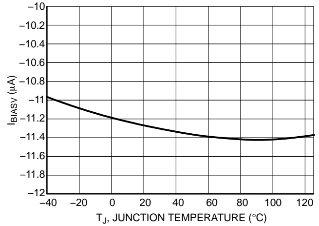
Figure 12. I_{BIASV} at V_{CC} = 15\text{ V} , V_{SNS} > V_{SNSBIASTH}
