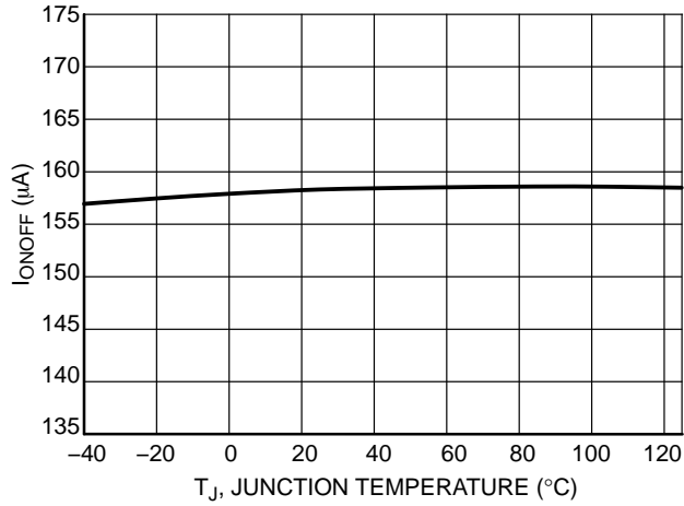
Figure 11. I_{ONOFF} at V_{CC} = 15\text{ V}
