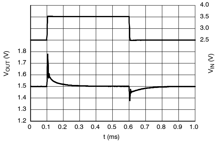
Figure 23. Line Transients, 1.5 V Version, t_R = t_F = 5\text{ }\mu\text{s} , I_{OUT} = 30\text{ mA}
