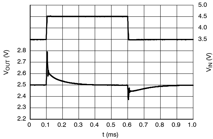
Figure 24. Line Transients, 2.5 V Version, t_R = t_F = 5\text{ }\mu\text{s} , I_{OUT} = 30\text{ mA}
