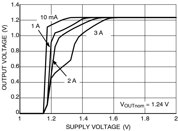
Figure 6. Dropout Characteristics
