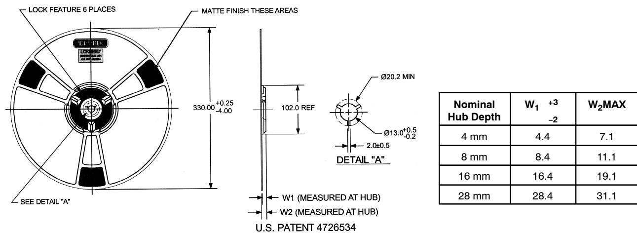
Figure 13. Reel Dimensions
