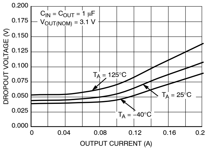
Figure 25. Dropout Voltage vs. Output Current V_{OUT} = 3.1\ \text{V}
