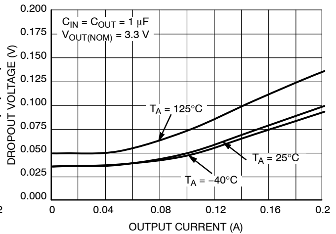
Figure 26. Dropout Voltage vs. Output Current V_{OUT} = 3.3\ \text{V}
