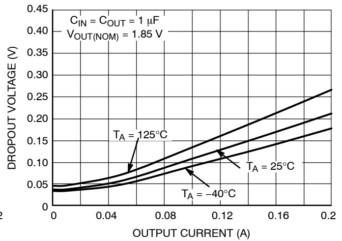
Figure 22. Dropout Voltage vs. Output Current V_{OUT} = 1.85\ \text{V}
