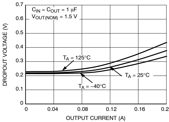
Figure 21. Dropout Voltage vs. Output Current V_{OUT} = 1.5\ \text{V}
