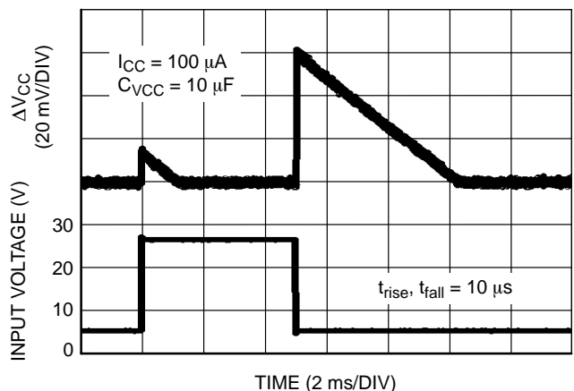
Figure 9. Line Transient Response ( V_{BB} 5 V to 26 V)
