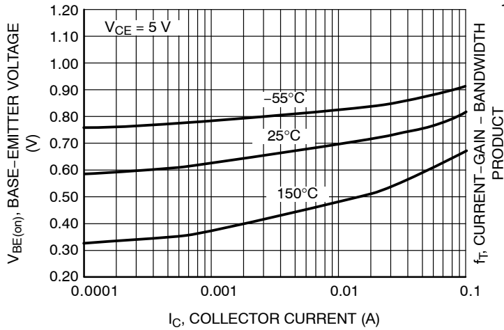
Figure 7. V_{BE(on)} at V_{CE} = 5\text{ V}
