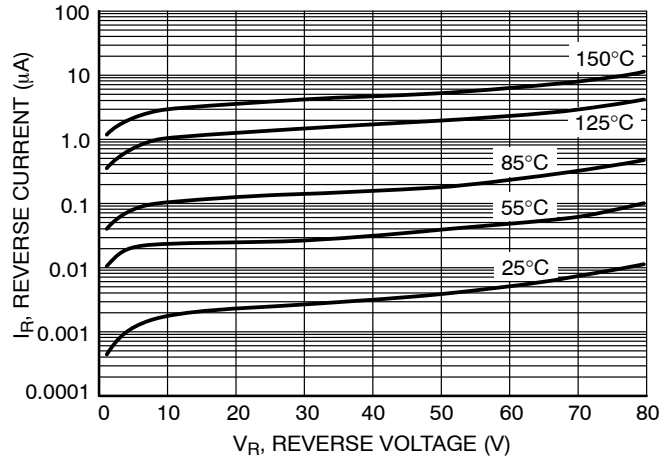
Figure 2. Reverse Current
