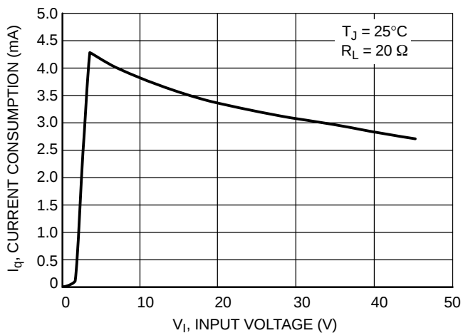
Figure 21. Current Consumption vs. Input Voltage, Adjustable Version
