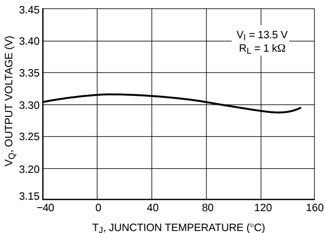
Figure 9. Output Voltage vs. Junction Temperature, 3.3 V Version
