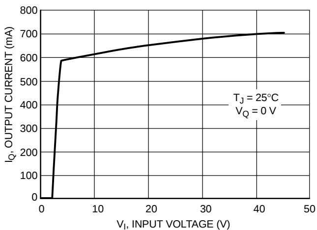
Figure 25. Maximum Output Current vs. Input Voltage, Adjustable Version
