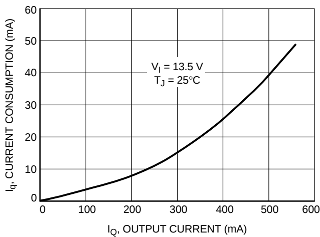
Figure 18. Current Consumption vs. Output Current (High Load)
