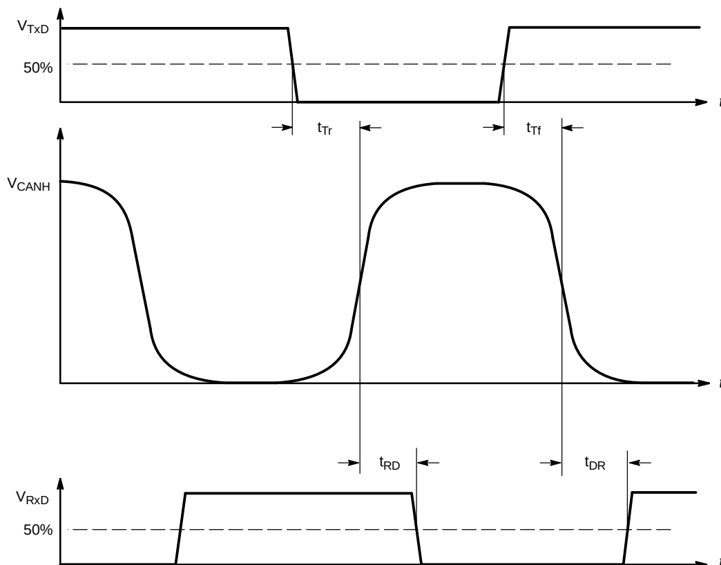
Figure 6. Input/Output Timing
