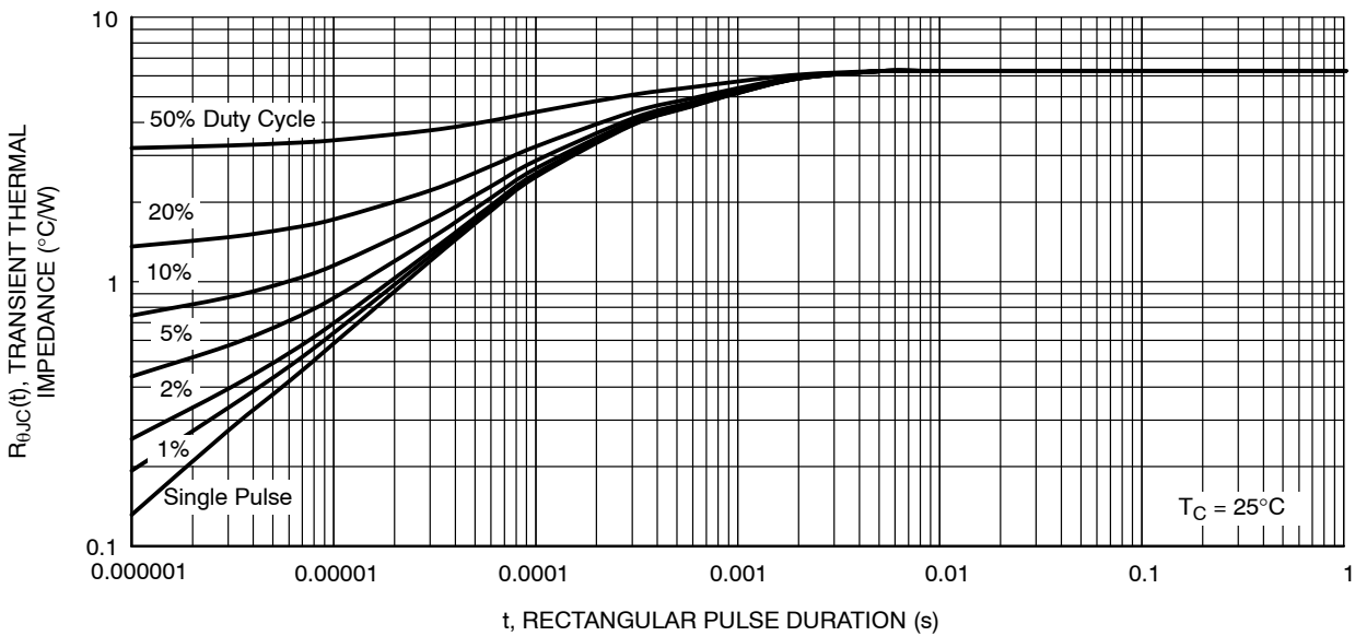
Figure 14. Thermal Response
