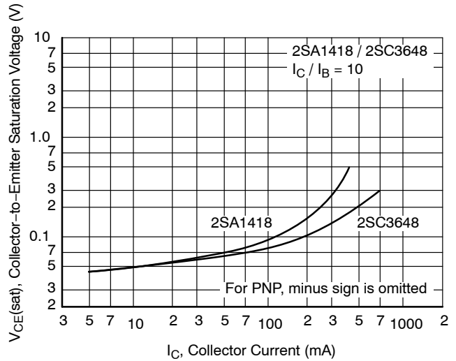
Figure 7. V_{CE(sat)} - I_C
