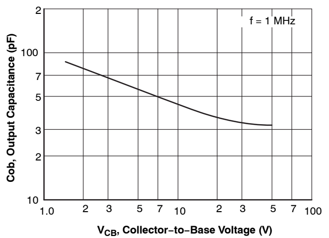
Figure 7. C_{ob} - V_{CB}
