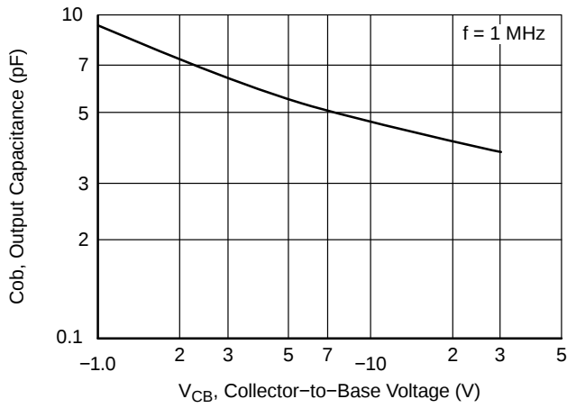
Figure 8. C_{ob} - V_{CB}
