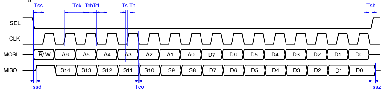
Figure 4. SPI 8 Bit Read/Write Access with Timing
