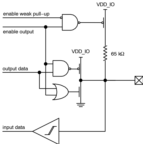
Figure 3. GPIO Pin
