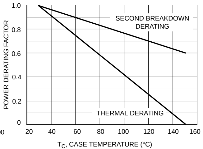
Figure 16. Power Derating
