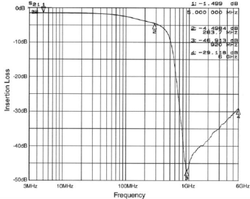
Figure 4. Insertion Loss vs. Frequency (A4-C4 to GND B2)
