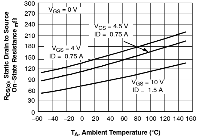
Figure 5. R_{DS(on)} - T_A
