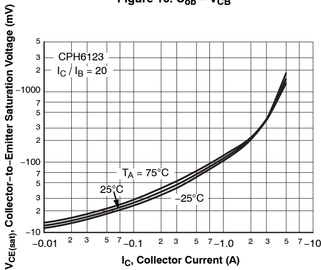
Figure 12. V_{CE(sat)} - I_C
