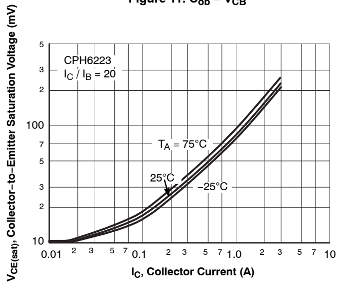
Figure 13. V_{CE(sat)} - I_C
