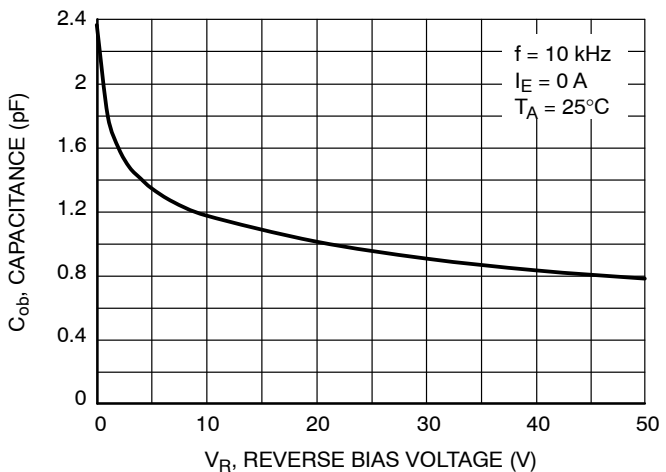
Figure 14. Output Capacitance
