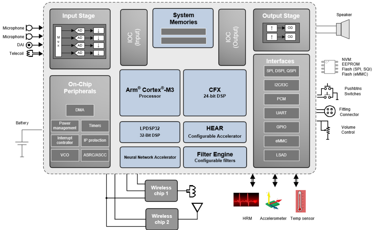
Figure 1. Ezairo 8300 Architecture
