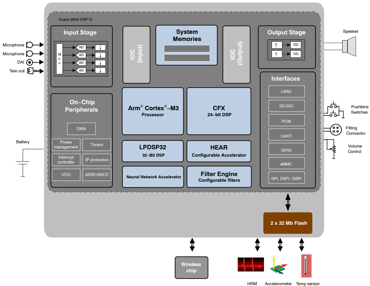
Figure 1. Ezairo 8510 Hybrid System Diagram
