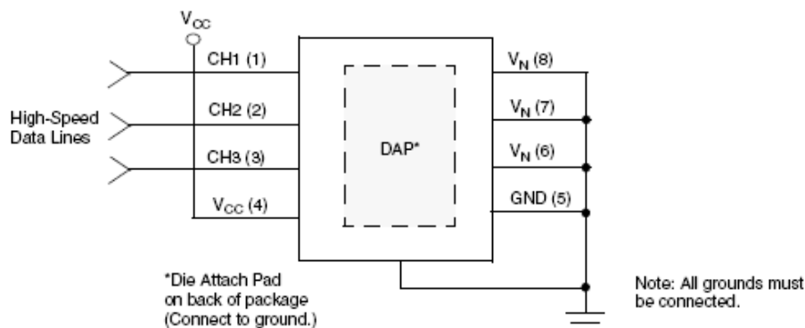
Figure 2. Typical Application
