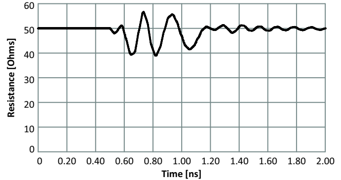
Figure 16. TDR - ESD8040
