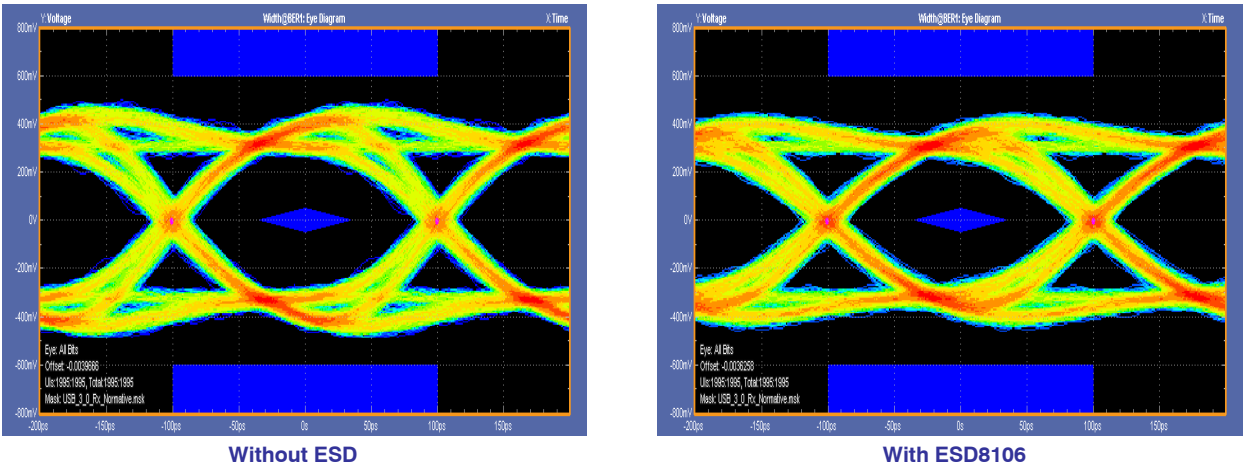
Figure 5. USB 3.0 Eye Diagram with and without ESD8106. 5.0 Gb/s, 400 mV pp
