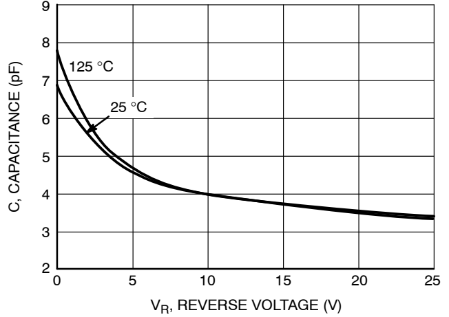
Figure 3. CV Characteristics
