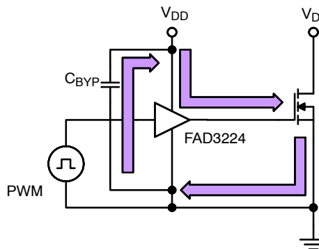
Figure 25. Current Path for MOSFET Turn-On
