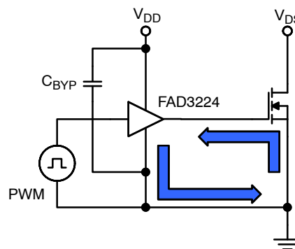
Figure 26. Current Path for MOSFET Turn-Off
