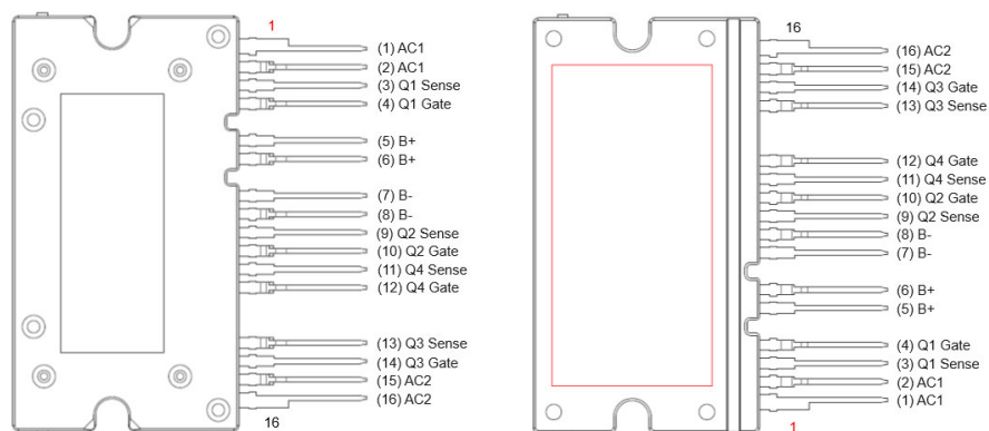
Figure 1. Pin Configuration
