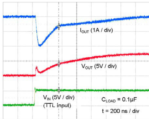
Figure 45. Quasi-Static Source Current with V_{DD} = 8\text{ V}
