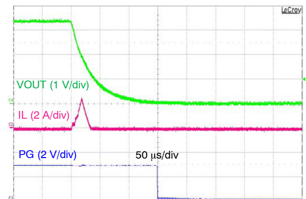
Figure 34. Output Fault, V_{IN} = 3.0\text{ V} , V_{OUT} = 3.3\text{ V}
