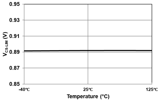
Figure 15. Current Limit Threshold Voltage (V CS-LIM ) vs. Temperature
