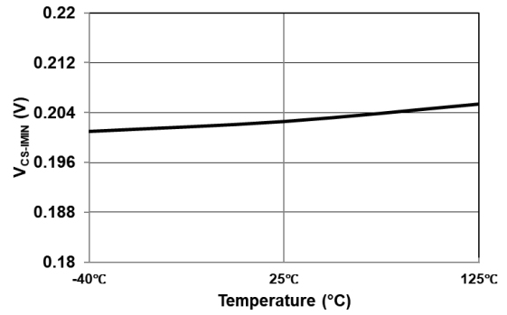
Figure 16. Current Sense Threshold Voltage (V CS-IMIN ) vs. Temperature
