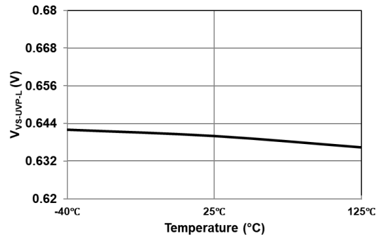
Figure 18. Output Under-Voltage Protection with VS Sampling Voltage (V VS-OVP-L ) vs. Temperature
