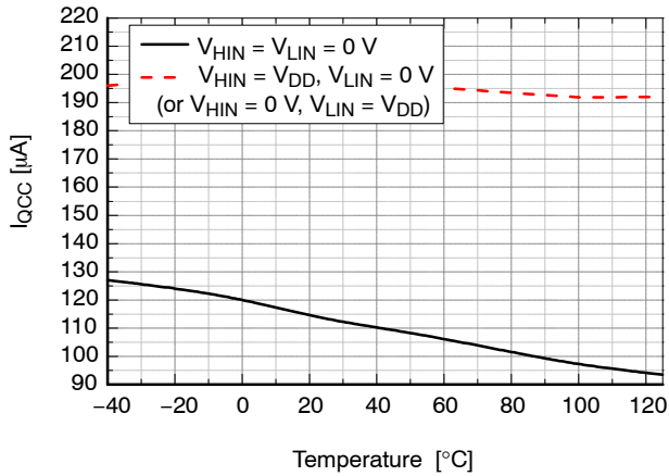
Figure 12. Quiescent V CC Supply Current
