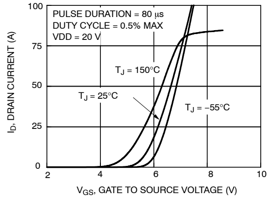
Figure 6. Transfer Characteristics
